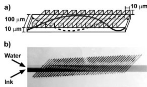
Fig. 4. a) Schematic diagram of the twisting flow of two liquids (solid and dashed lines) in a microfluidic channel patterned with grooves on one face. The dimensions shown are those of the channel in (b). b) Optical micrograph of two streams of liquids (water (light) and ink (dark)) as they flow axially through the channel. The dark lines, oriented 45^\circ to the long axis of the channel, are grooves in the top of the channel. The grooves extend beyond the length of the channel and these regions are filled with stagnant fluid.
